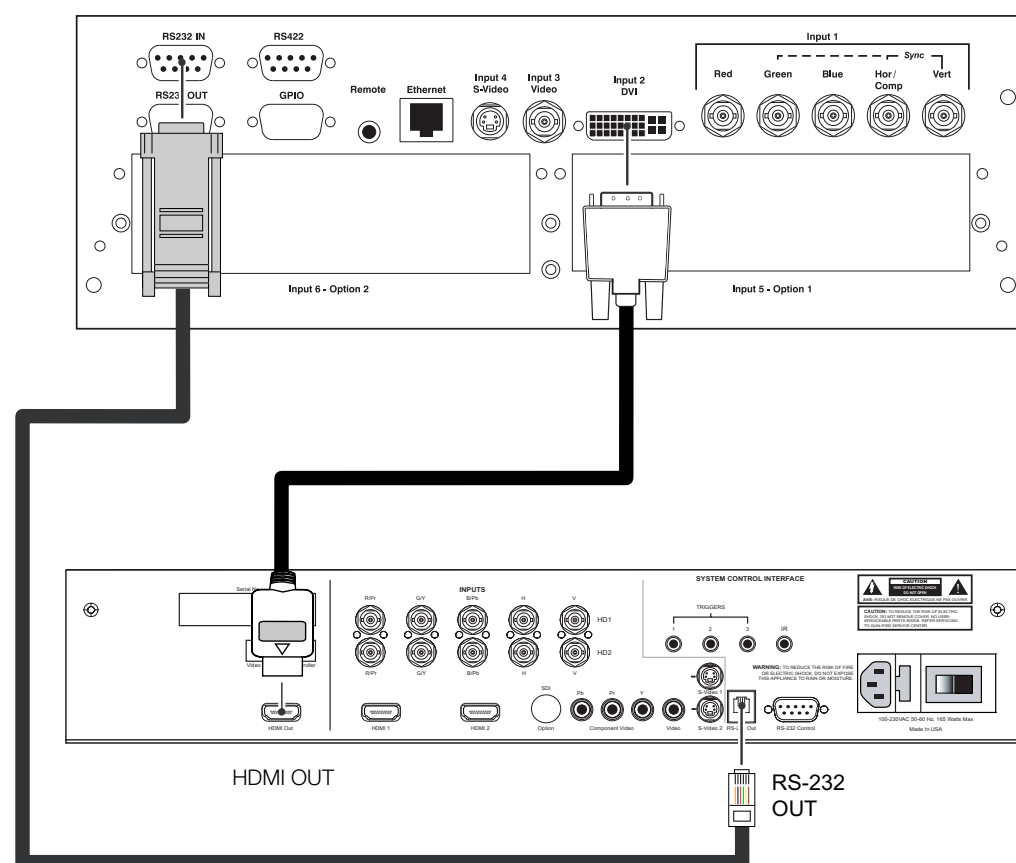
Figure 3-8. Connecting the VX-44d/-55d to the DHD Controller
